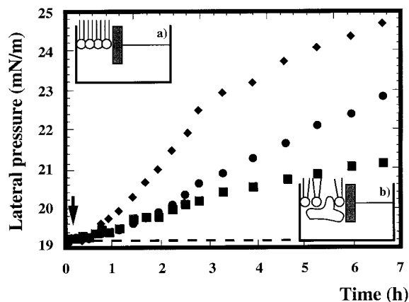
FIG. 2. A time/pressure diagram as measured by the film balance technique. Pure DMPG phospholipid monolayers were spread on buffer and 25 \mu\text{g/ml} GST (■), GST/49-71 (●), or GST/131-155 (◆) was injected into the subphase. The arrow marks the time of injection. The pressure of 19 mN/m was constant for pure DMPG (—) over 10 h. (Note: the equilibrium pressure reached after 15 h was 28.5, 25, and 21.5 mN/m for GST/131-155, GST/49-71, and GST, respectively). Measuring temperature 20°C. Buffer (A): 20 mM HEPES/NaOH pH 7.4, 0.3 mM EGTA, 0.3 mM EDTA, 0.2 mM DTT, 5 mM NaCl, 0.005% \text{NaN}_3 . (Inset: schematic representation of the film balance technique. Changes in pressure with time (a+b) are due to the insertion of the protein into the lipid layer).
